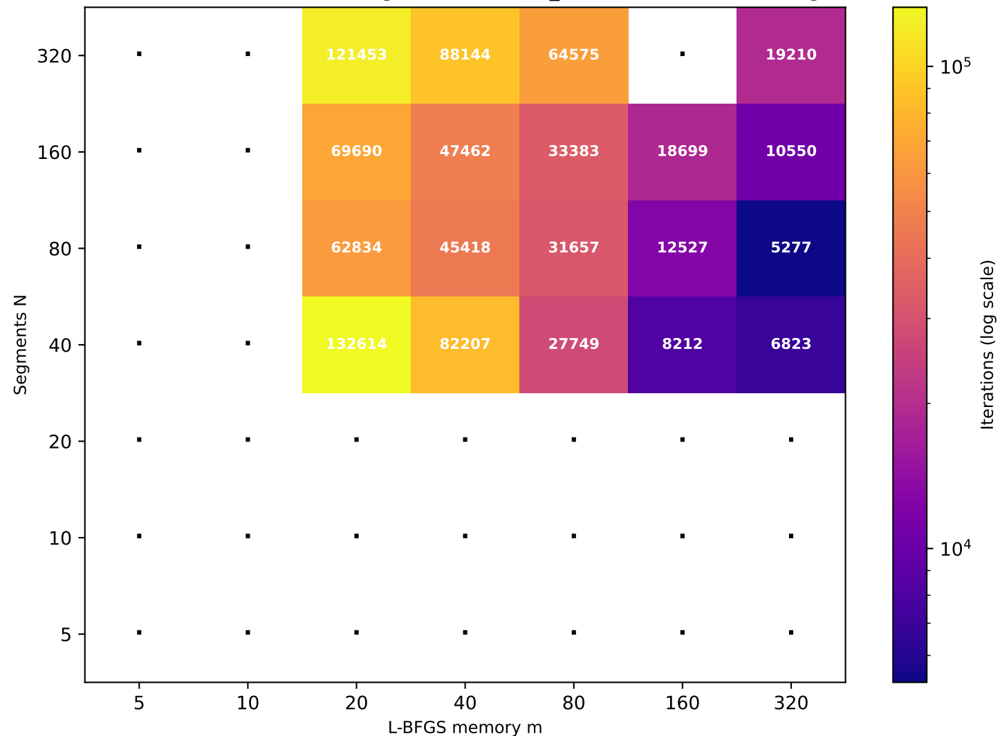
Recurrence T \approx 158.05 (target T=160 , rec_id=62) [19/49 converged]
