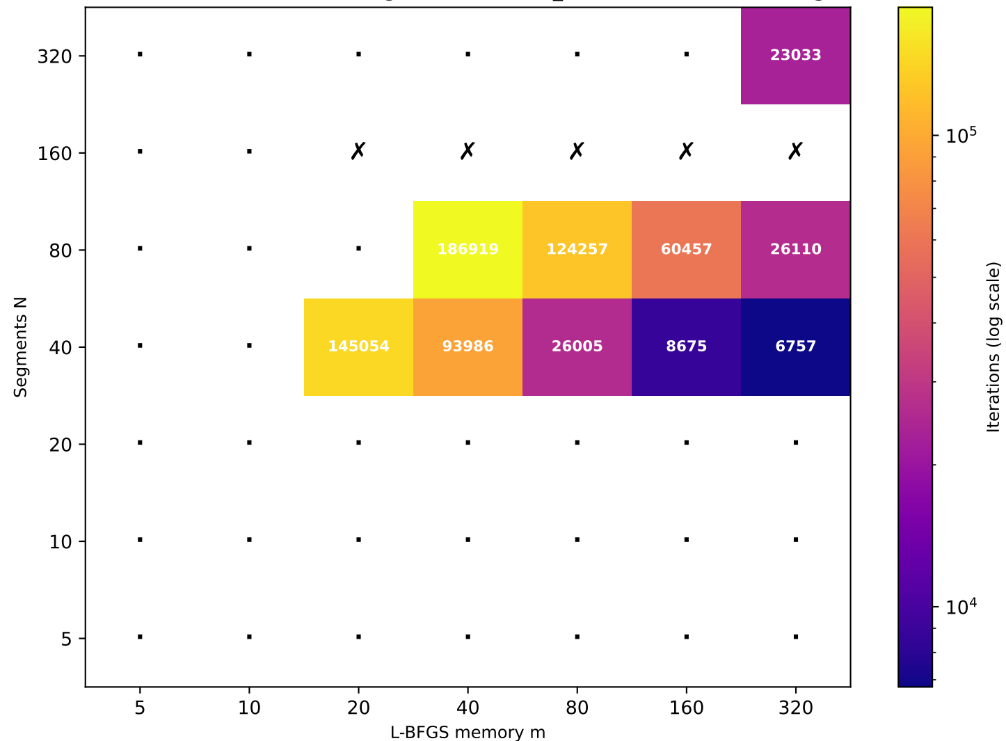
Recurrence T \approx 159.06 (target T=160 , rec_id=67) [10/49 converged]
