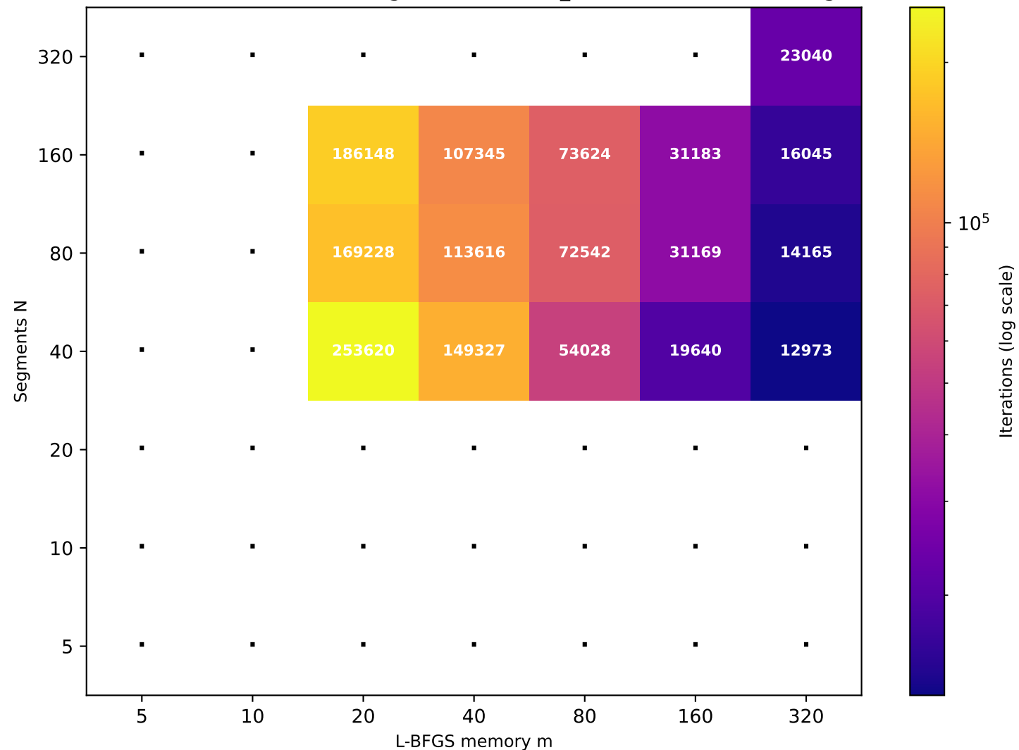
Recurrence T \approx 161.61 (target T=160 , rec_id=73) [16/49 converged]
