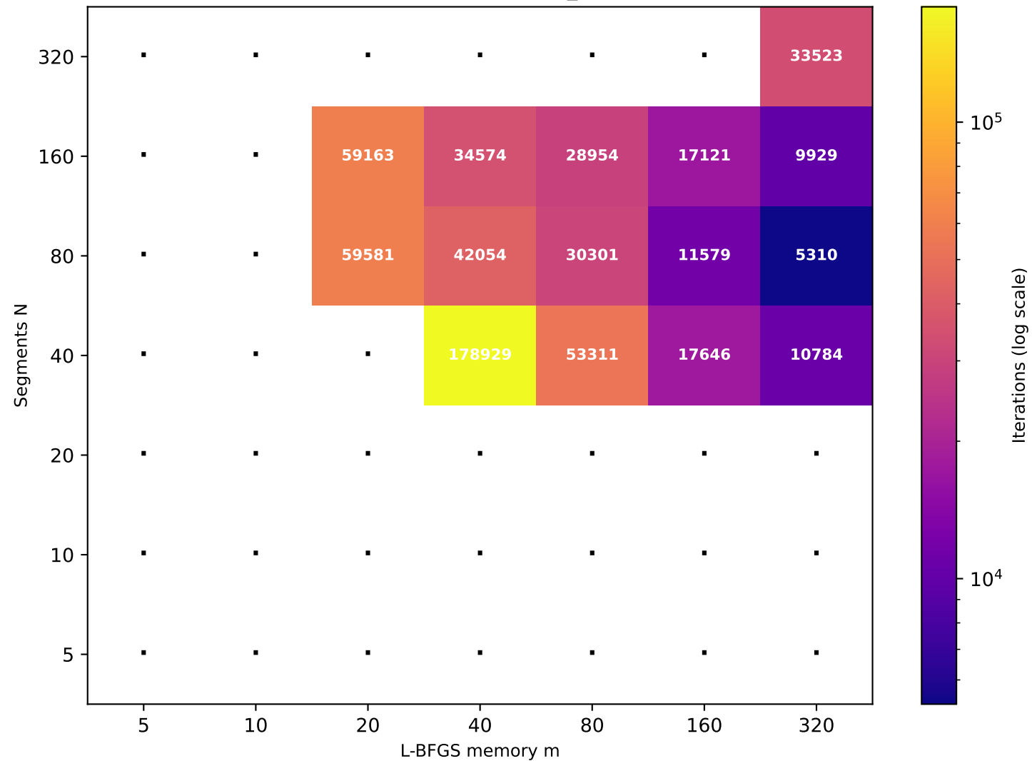
Recurrence T \approx 159.44 (target T=160 , rec_id=82) [15/49 converged]
