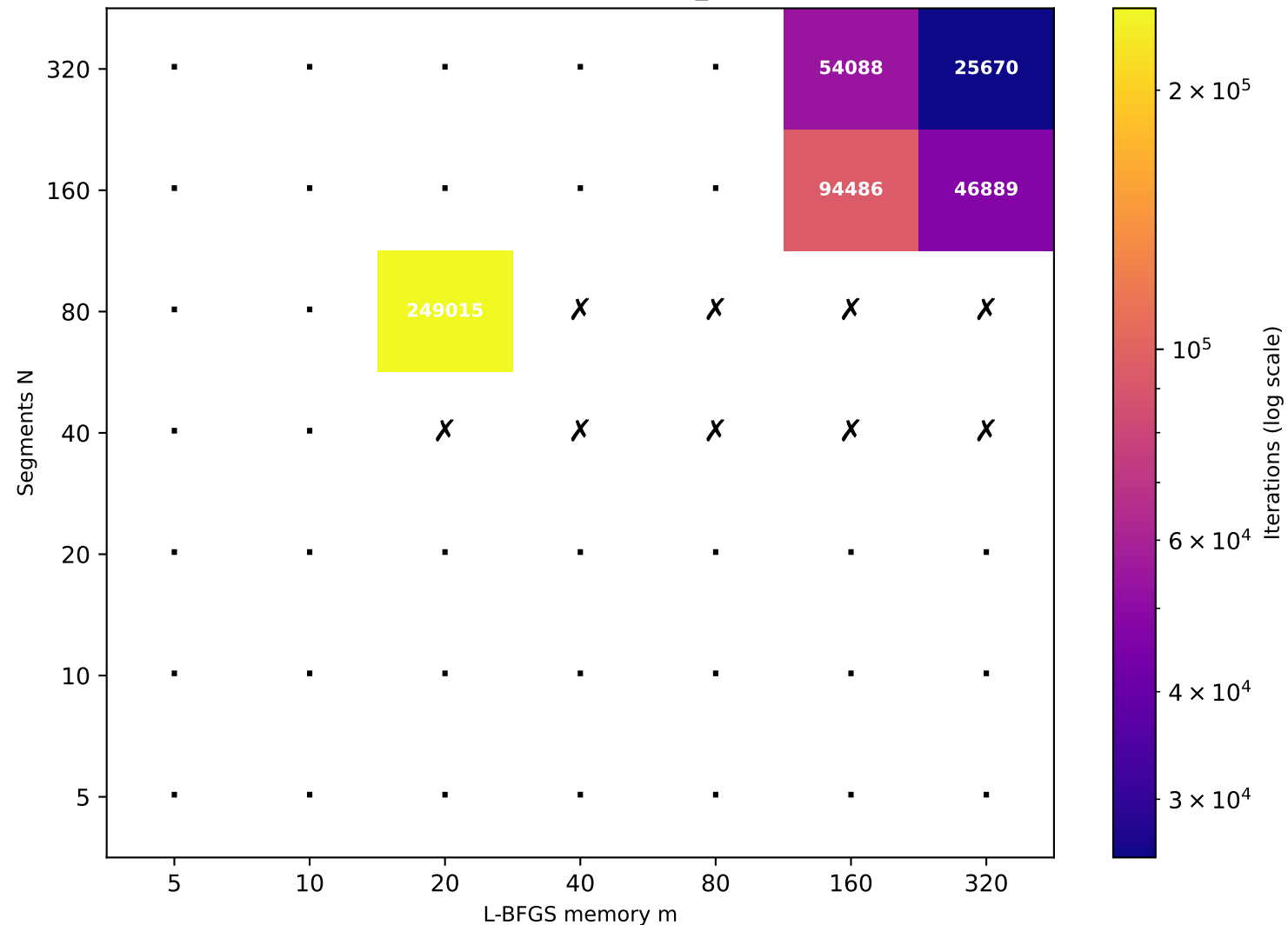
Recurrence T \approx 159.45 (target T=160 , rec_id=86) [5/49 converged]
