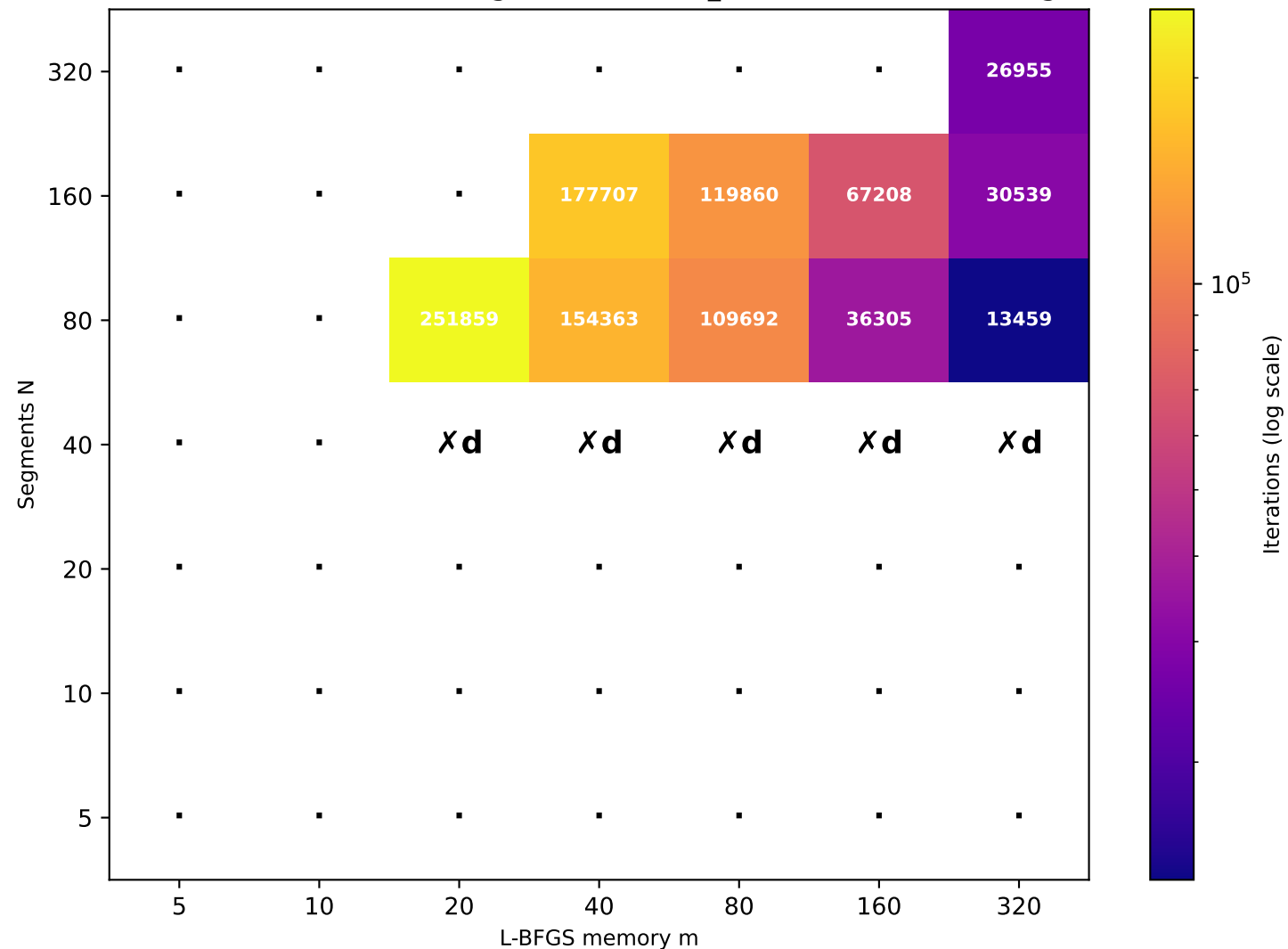
Recurrence T \approx 160.21 (target T=160 , rec_id=88) [10/49 converged]
