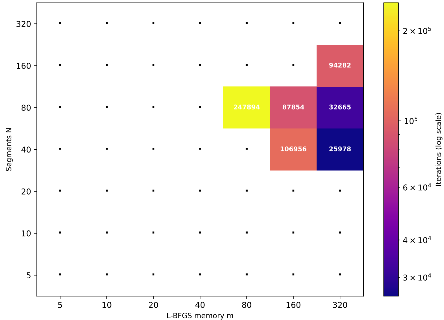
Recurrence T \approx 159.48 (target T=160 , rec_id=92) [6/49 converged]
