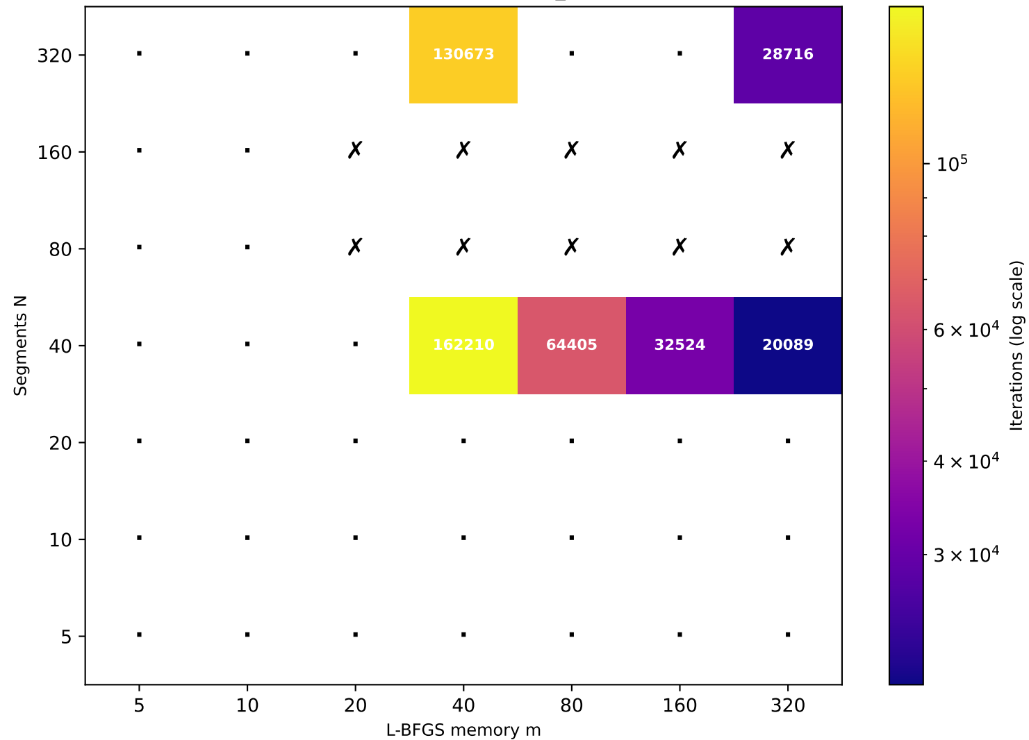
Recurrence T \approx 162.19 (target T=160 , rec_id=95) [6/49 converged]
