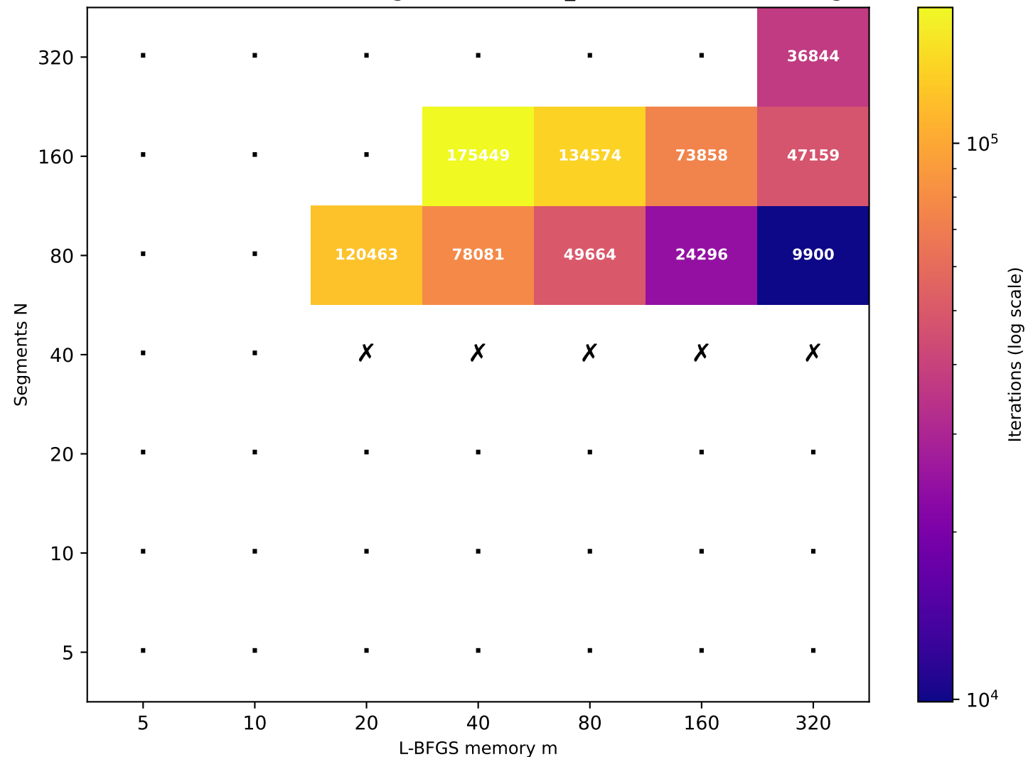
Recurrence T \approx 161.01 (target T=160 , rec_id=97) [10/49 converged]
