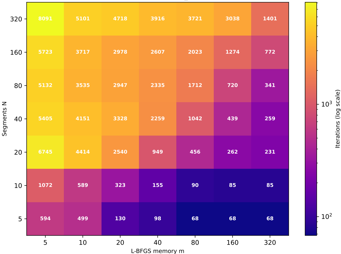
Recurrence T \approx 18.17 (target T=20 , rec_id=1) [49/49 converged]
