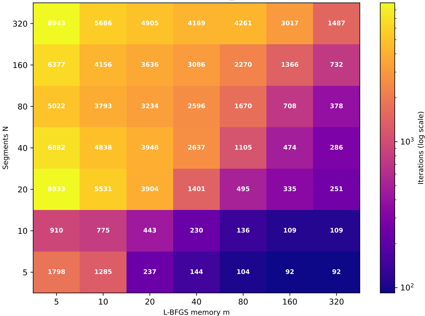
Recurrence T \approx 18.88 (target T=20 , rec_id=3) [49/49 converged]
