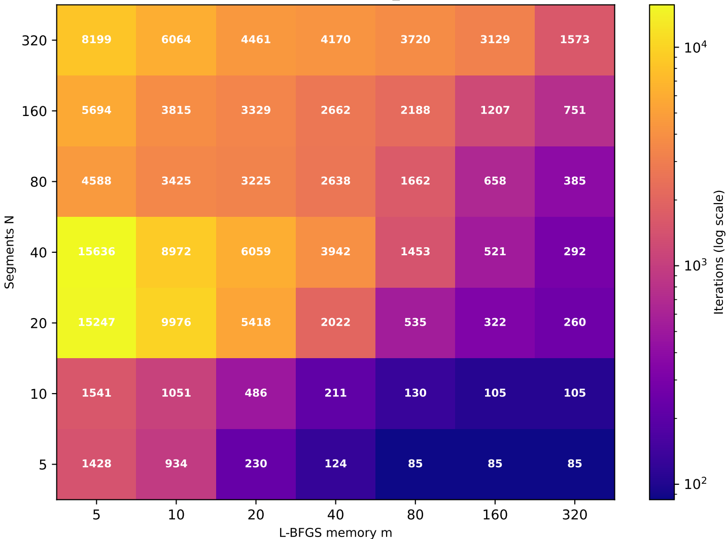
Recurrence T \approx 18.17 (target T=20 , rec_id=8) [49/49 converged]
