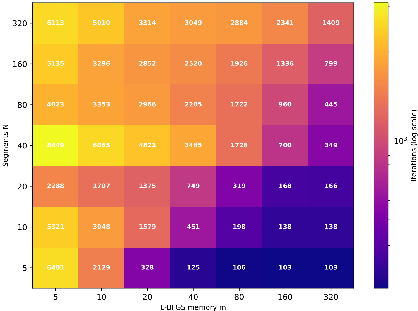
Recurrence T \approx 21.55 (target T=20 , rec_id=13) [49/49 converged]
