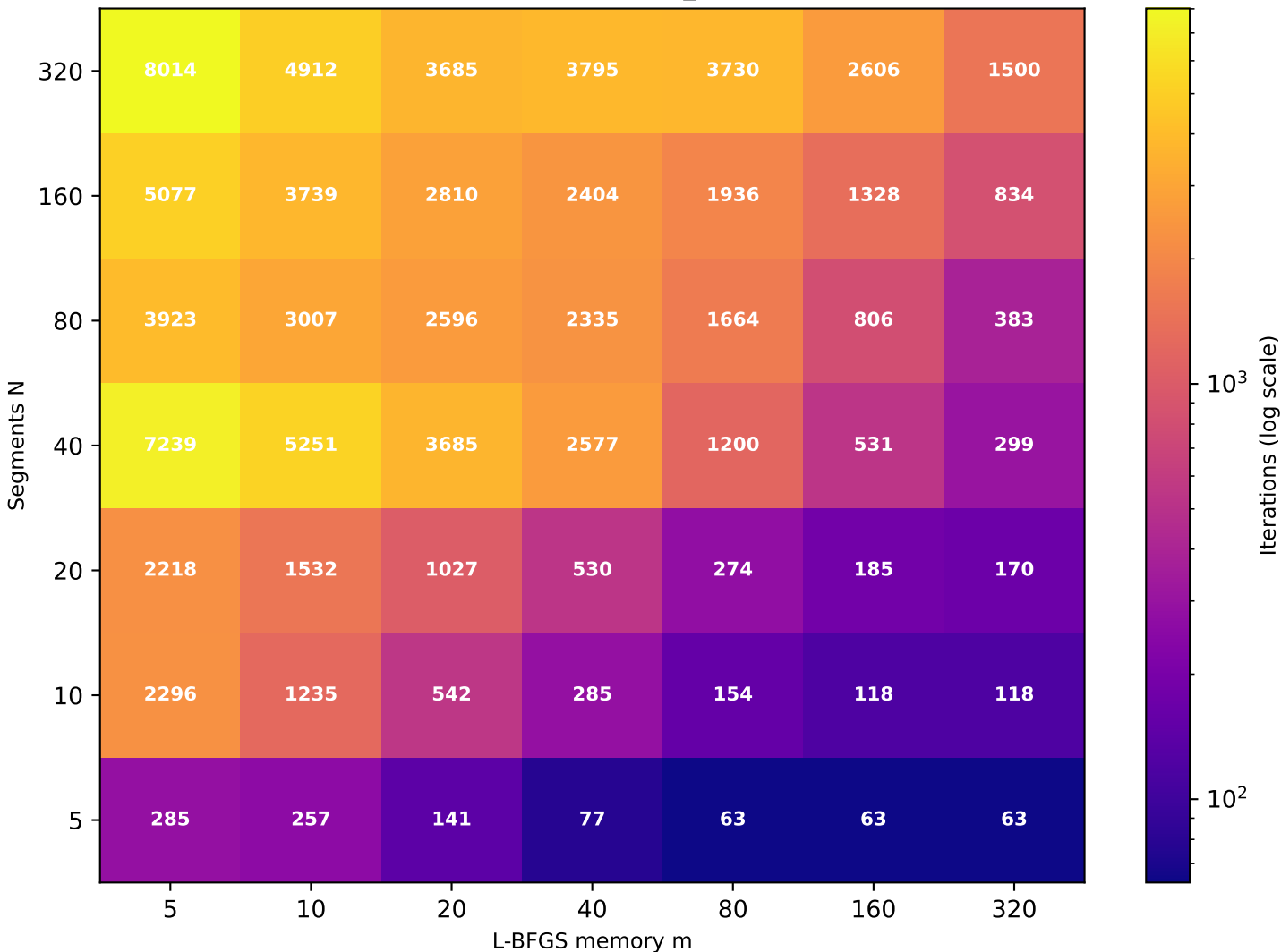
Recurrence T \approx 19.09 (target T=20 , rec_id=19) [49/49 converged]
