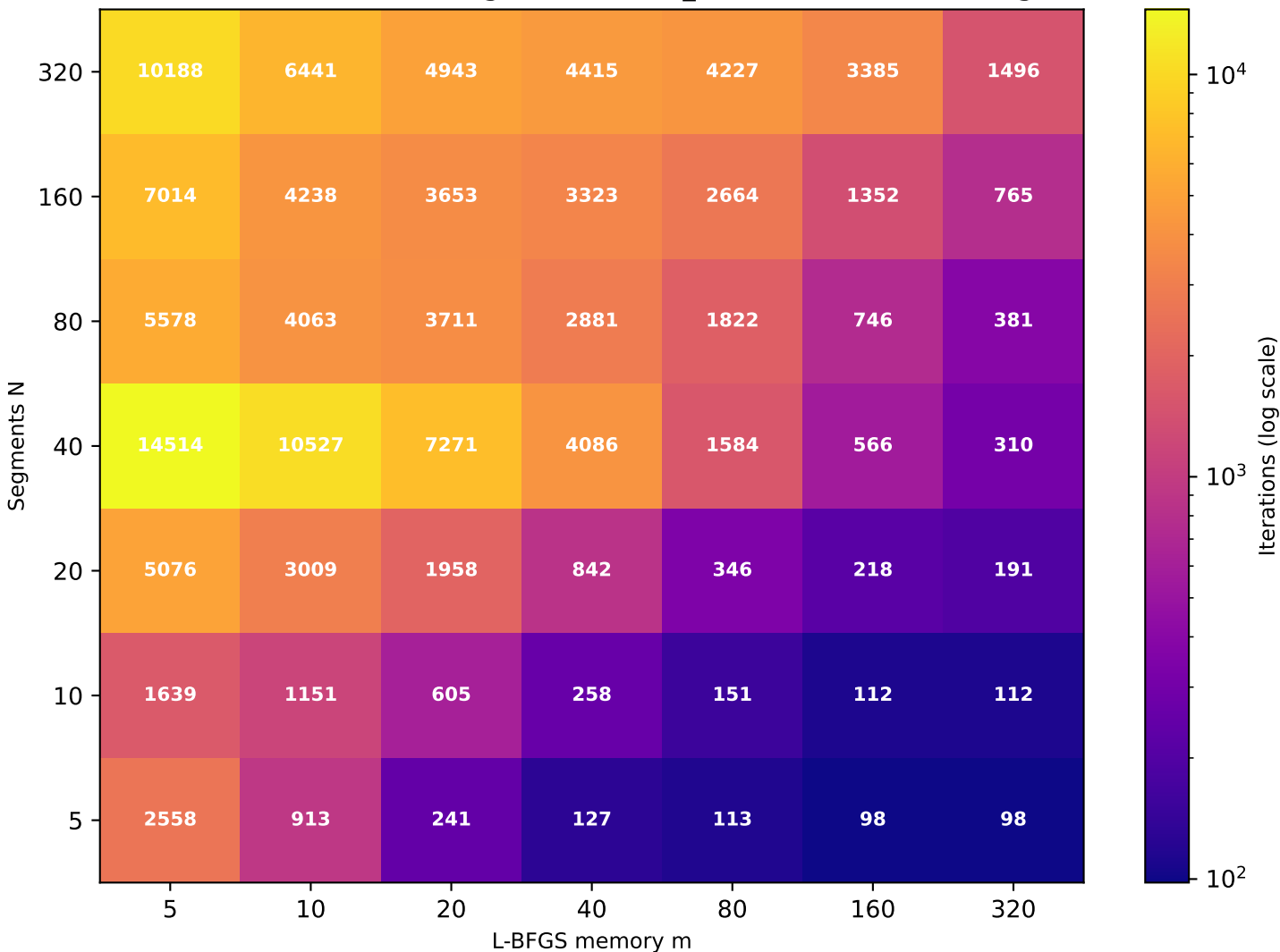
Recurrence T \approx 18.85 (target T=20 , rec_id=22) [49/49 converged]
