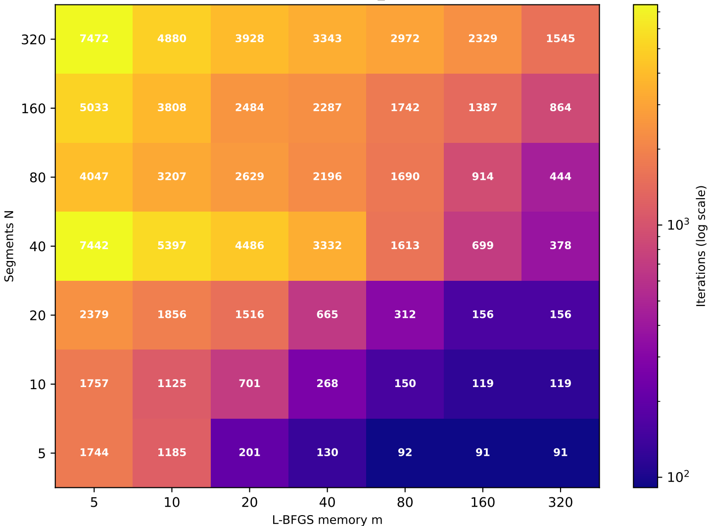
Recurrence T \approx 21.55 (target T=20 , rec_id=23) [49/49 converged]
