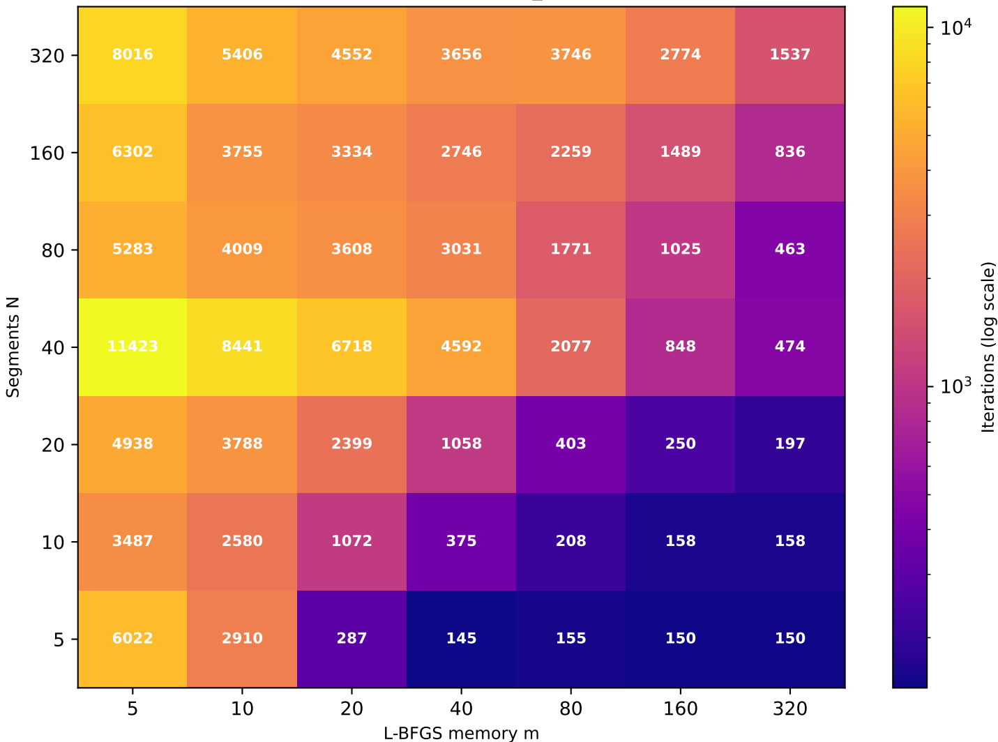
Recurrence T \approx 21.52 (target T=20 , rec_id=27) [49/49 converged]
