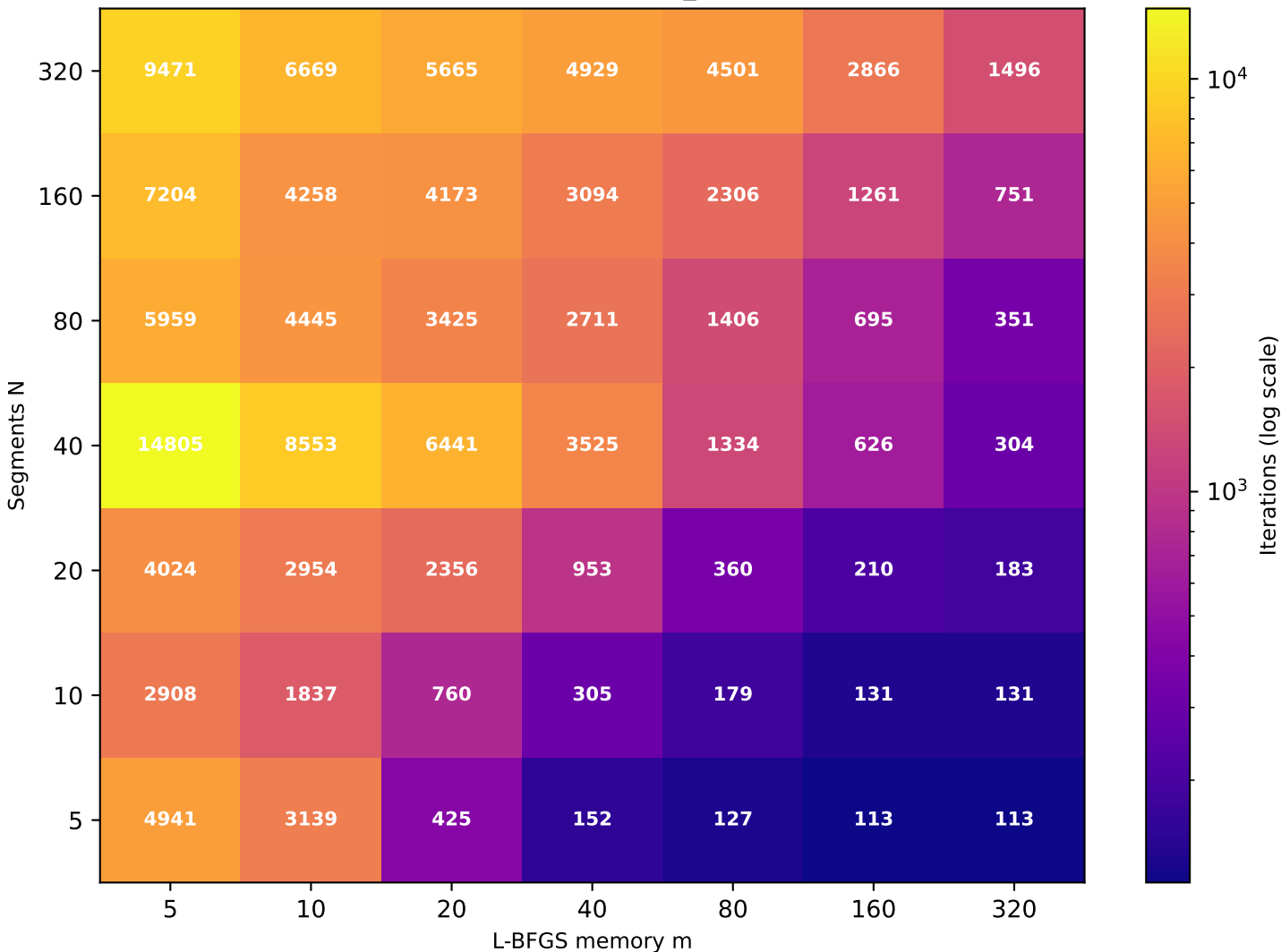
Recurrence T \approx 18.13 (target T=20 , rec_id=28) [49/49 converged]
