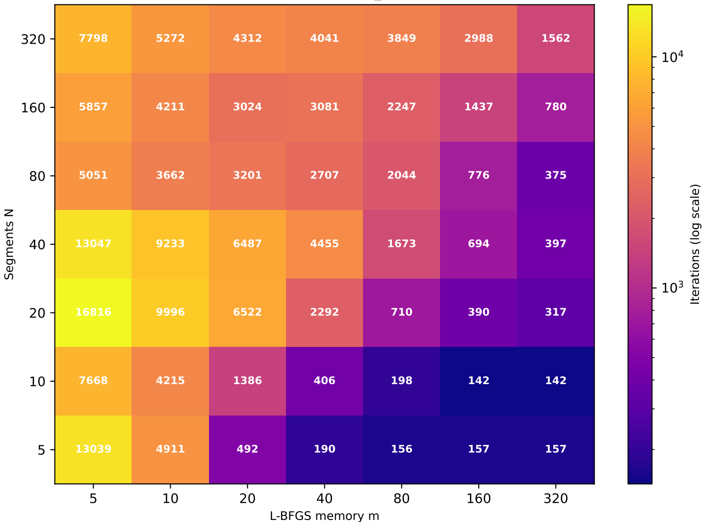
Recurrence T \approx 19.74 (target T=20 , rec_id=30) [49/49 converged]
