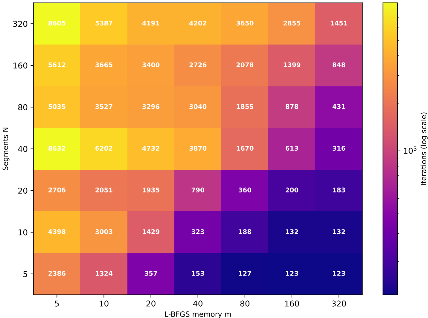
Recurrence T \approx 20.71 (target T=20 , rec_id=32) [49/49 converged]
