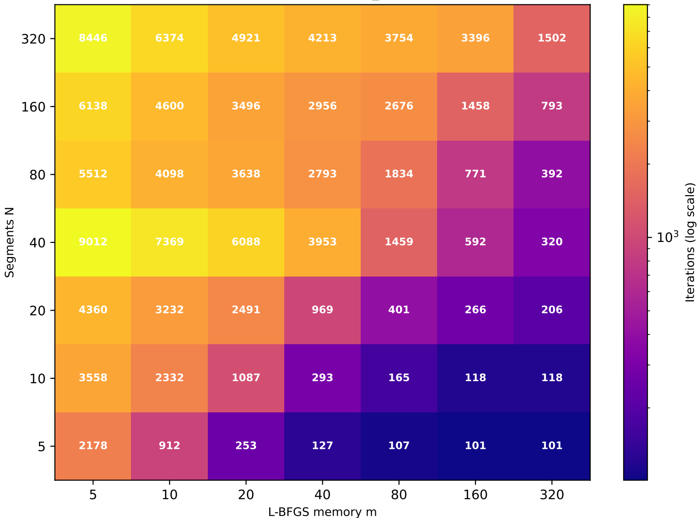
Recurrence T \approx 19.73 (target T=20 , rec_id=38) [49/49 converged]
