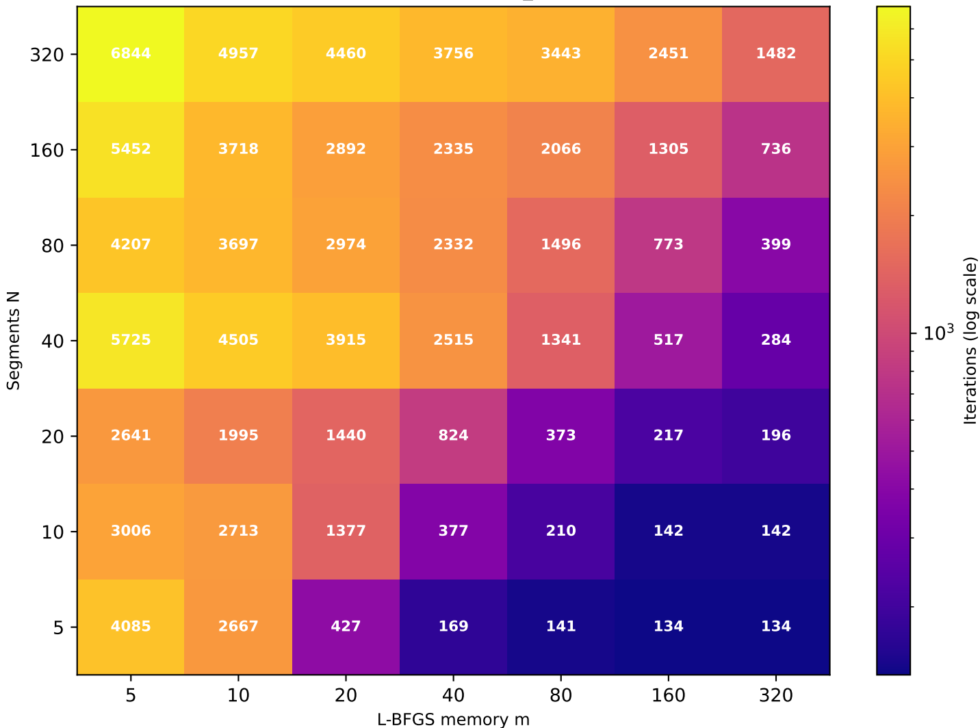
Recurrence T \approx 19.21 (target T=20 , rec_id=42) [49/49 converged]
