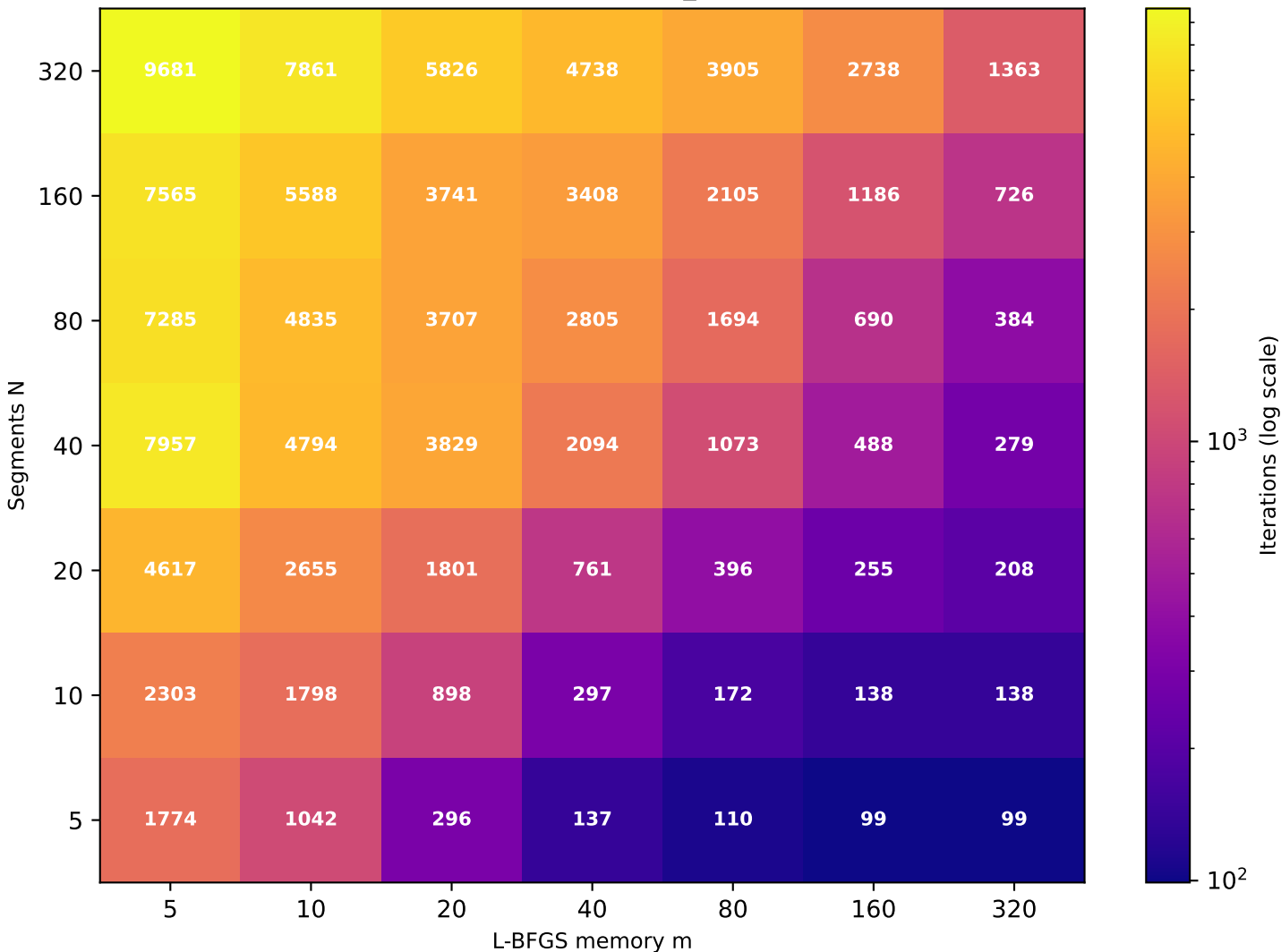
Recurrence T \approx 18.30 (target T=20 , rec_id=45) [49/49 converged]
