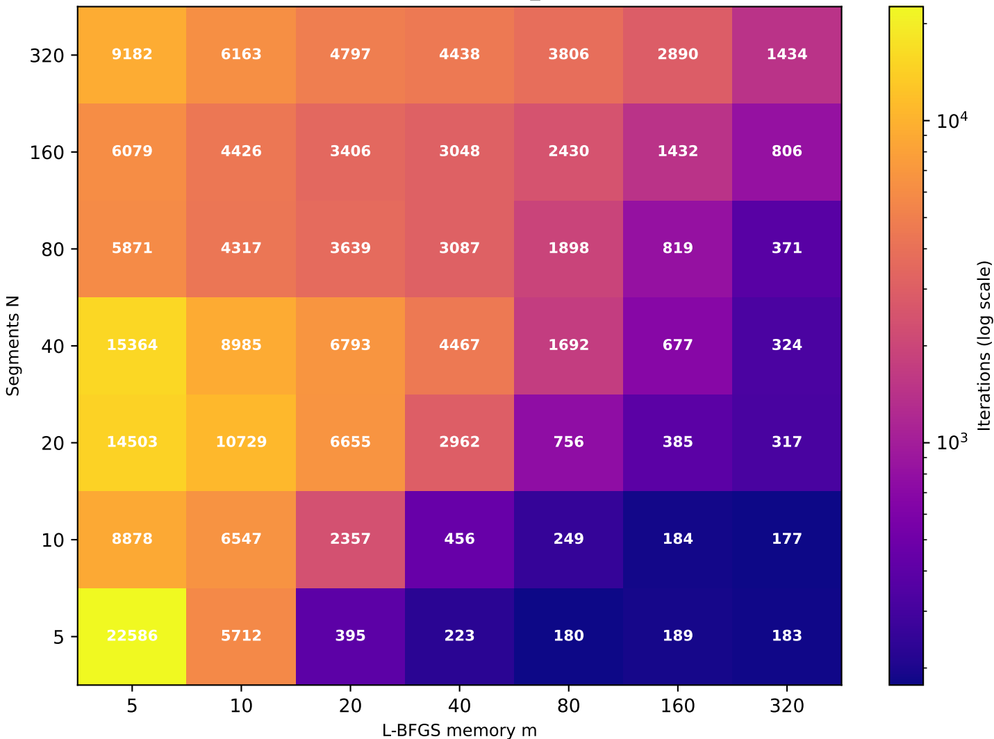
Recurrence T \approx 19.74 (target T=20 , rec_id=47) [49/49 converged]
