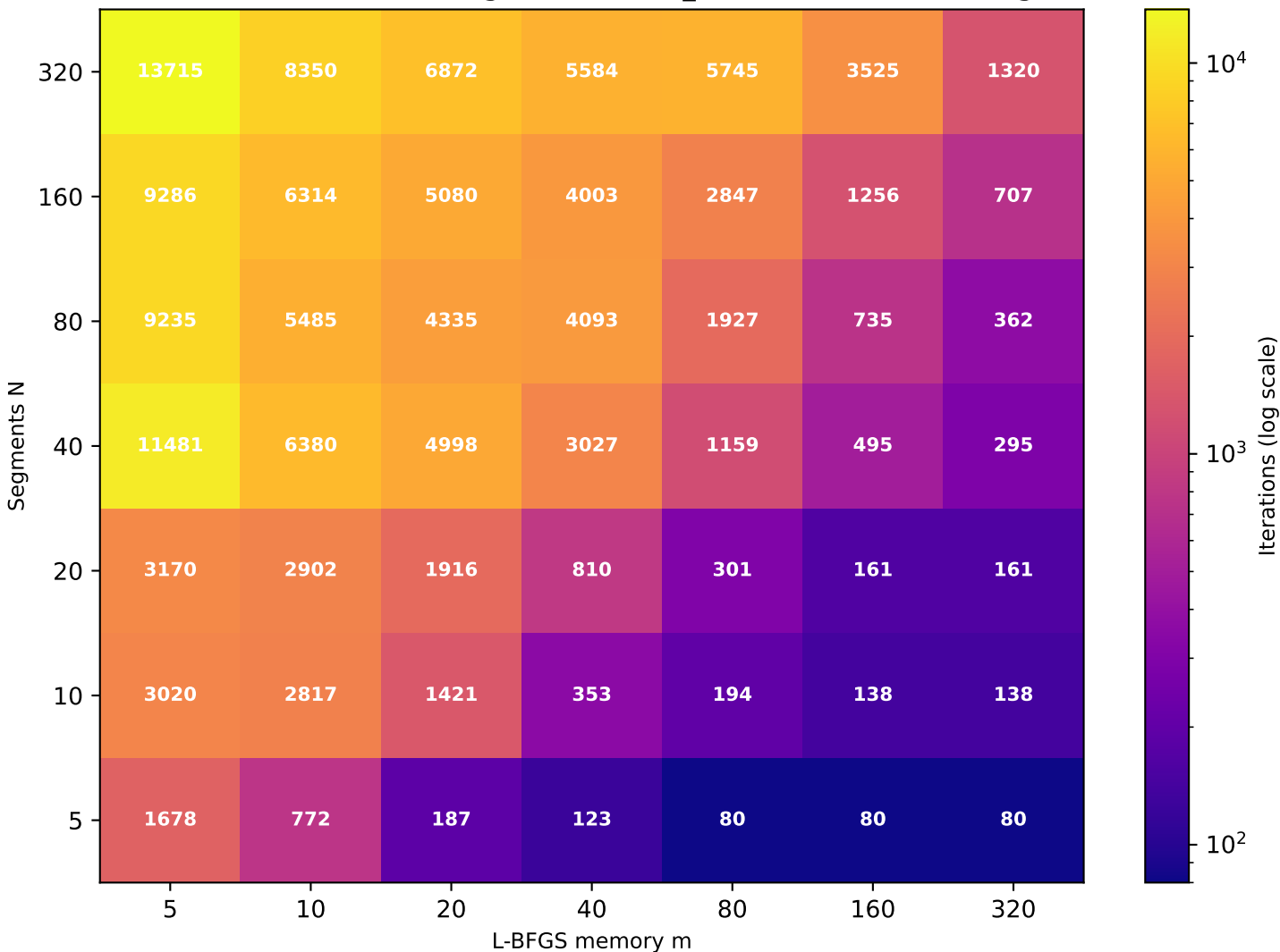
Recurrence T \approx 18.77 (target T=20 , rec_id=55) [49/49 converged]
