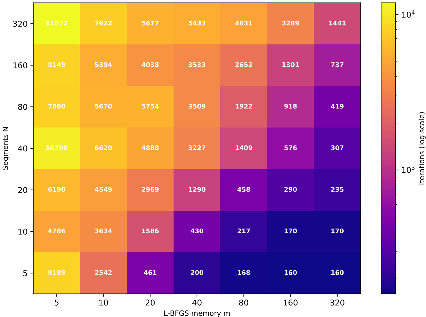
Recurrence T \approx 20.58 (target T=20 , rec_id=56) [49/49 converged]
