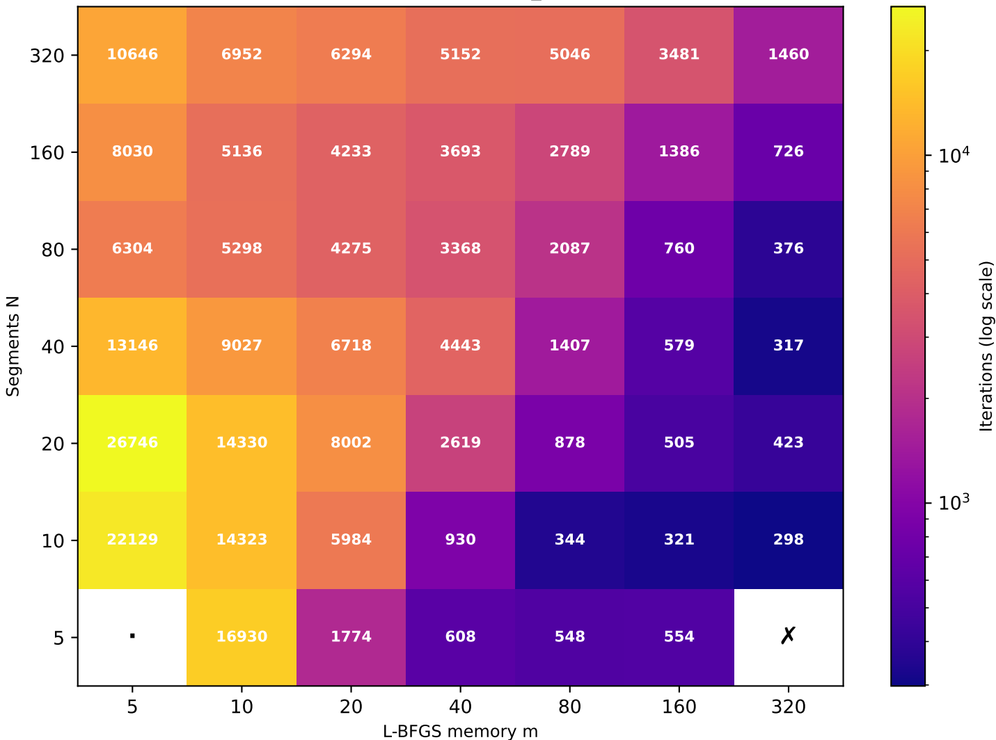
Recurrence T \approx 20.27 (target T=20 , rec_id=58) [47/49 converged]
