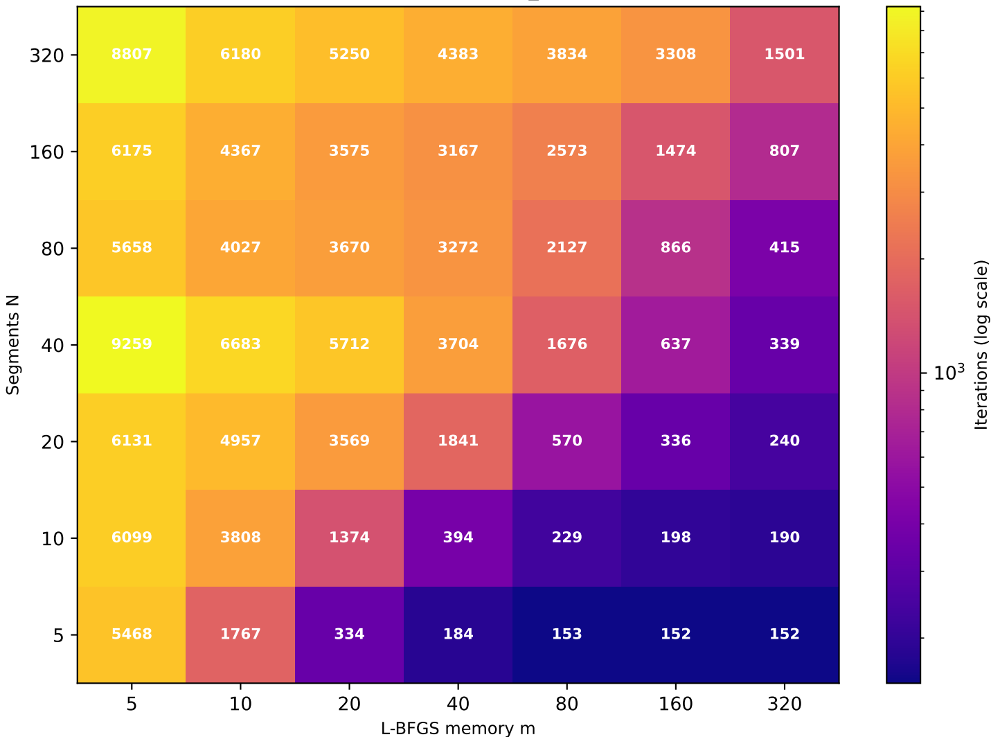
Recurrence T \approx 20.63 (target T=20 , rec_id=59) [49/49 converged]
