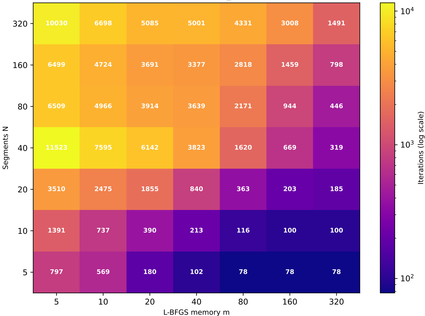
Recurrence T \approx 21.30 (target T=20 , rec_id=62) [49/49 converged]
