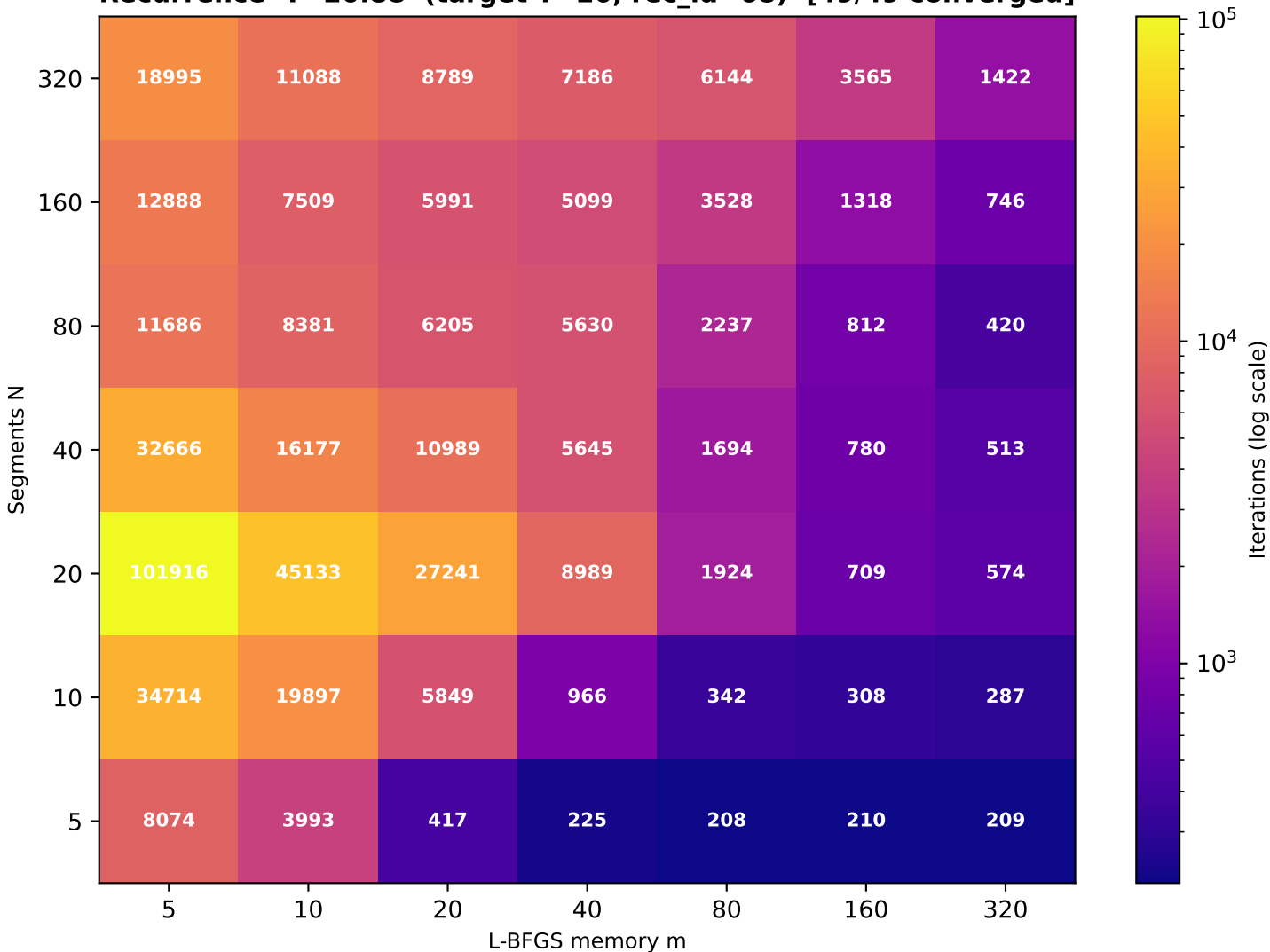
Recurrence T \approx 20.88 (target T=20 , rec_id=68) [49/49 converged]
