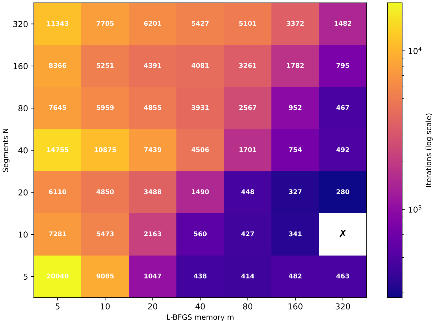
Recurrence T \approx 21.89 (target T=20 , rec_id=71) [48/49 converged]
