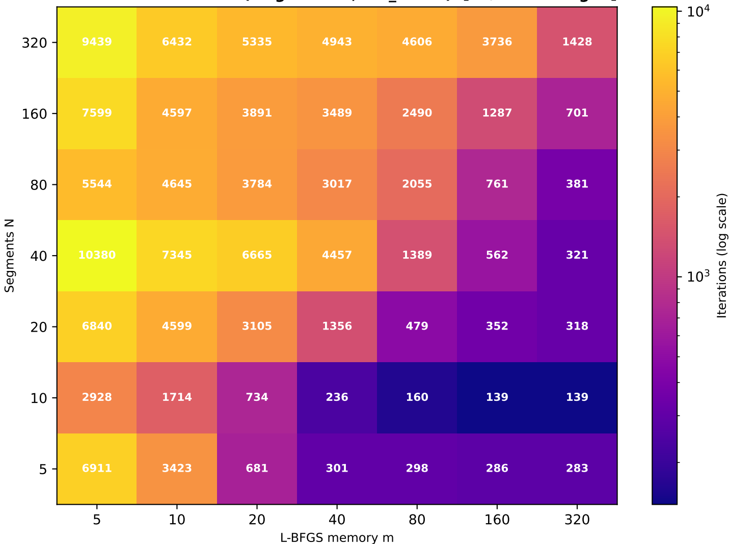
Recurrence T \approx 18.99 (target T=20 , rec_id=86) [49/49 converged]
