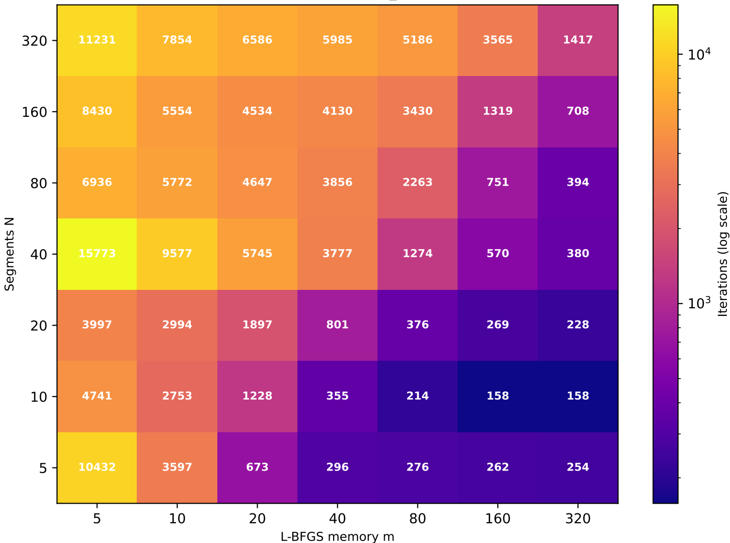
Recurrence T \approx 19.55 (target T=20 , rec_id=87) [49/49 converged]
