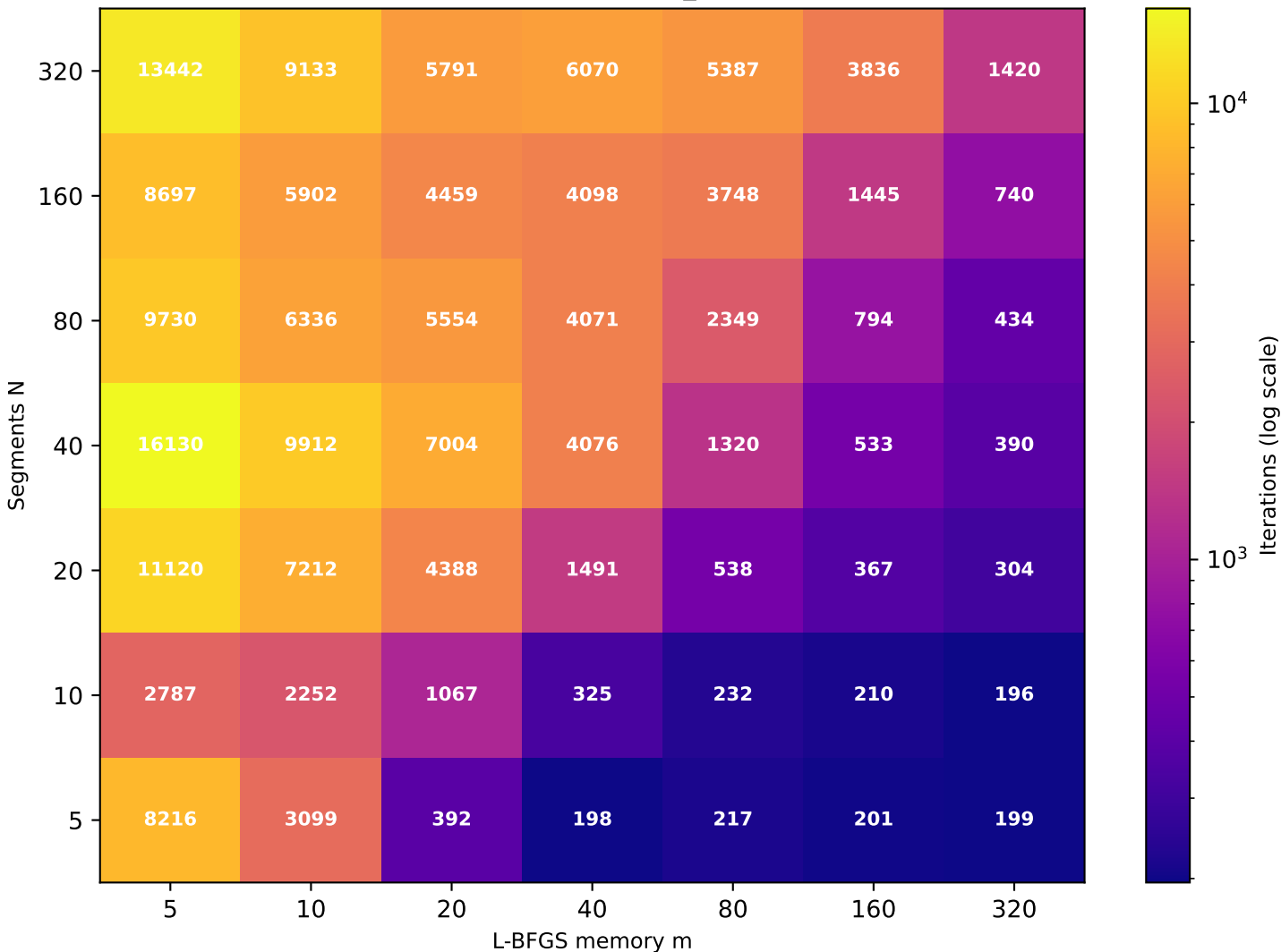
Recurrence T \approx 20.99 (target T=20 , rec_id=89) [49/49 converged]
