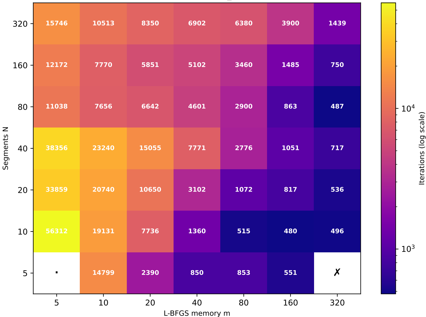
Recurrence T \approx 21.81 (target T=20 , rec_id=90) [47/49 converged]
