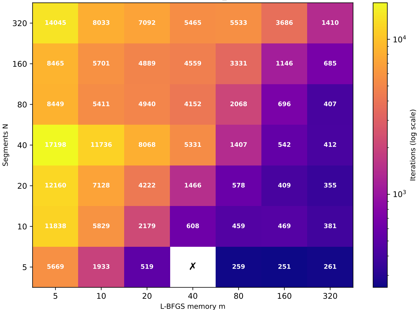
Recurrence T \approx 18.70 (target T=20 , rec_id=93) [48/49 converged]
