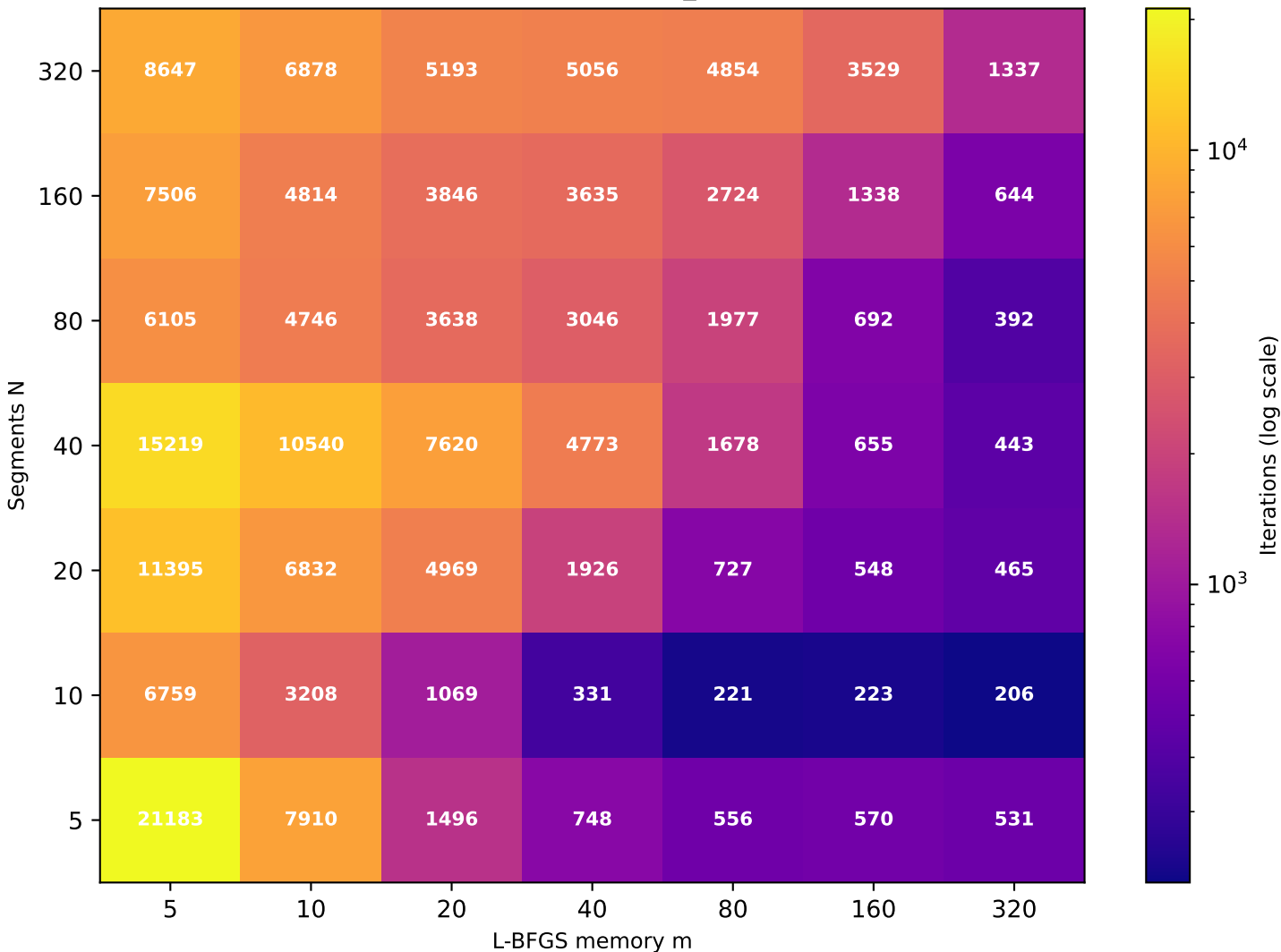
Recurrence T \approx 19.06 (target T=20 , rec_id=94) [49/49 converged]
