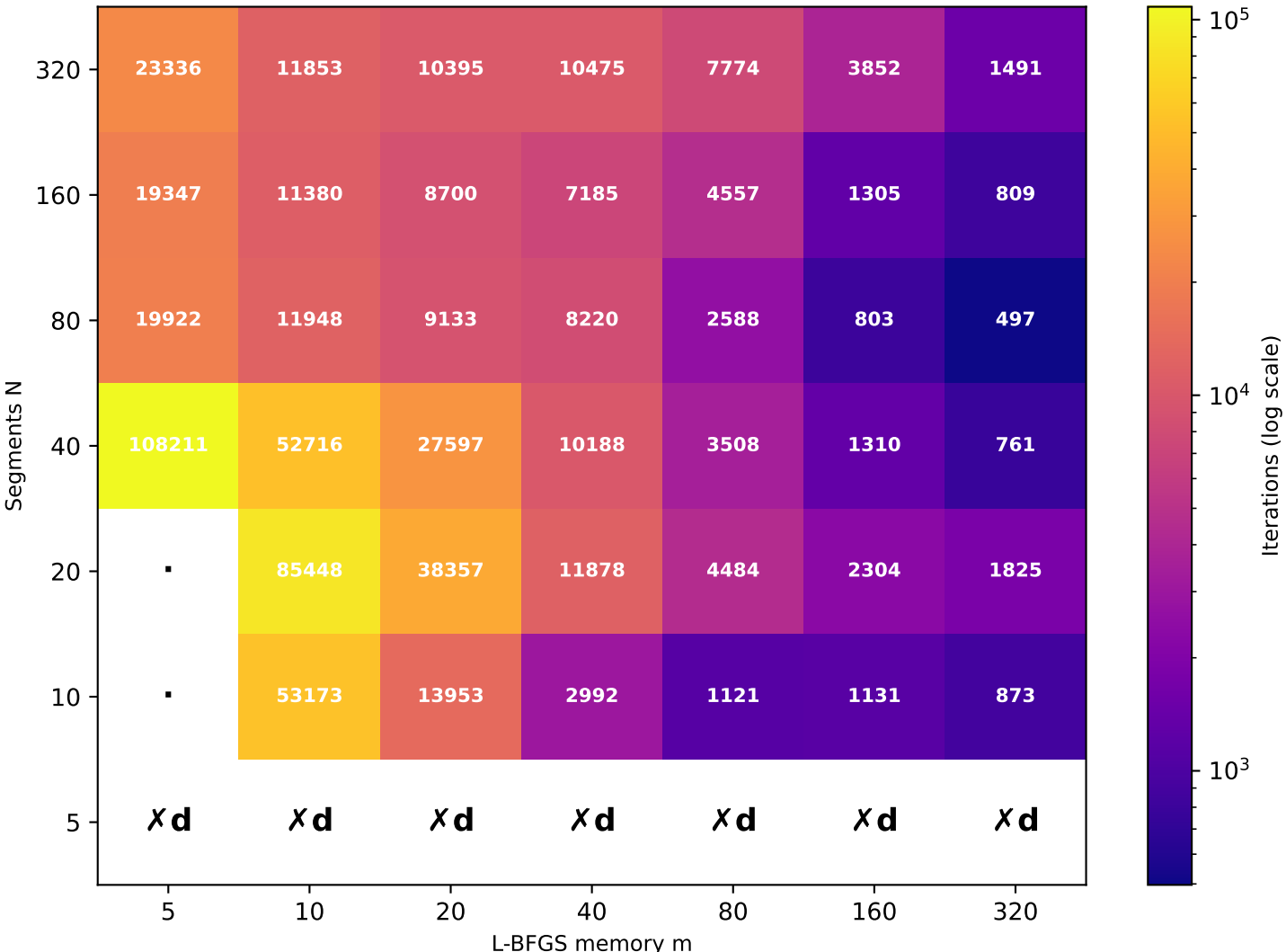
ecurrence T \approx 21.20 (target T=20, rec id=96) [40/49 converged]
