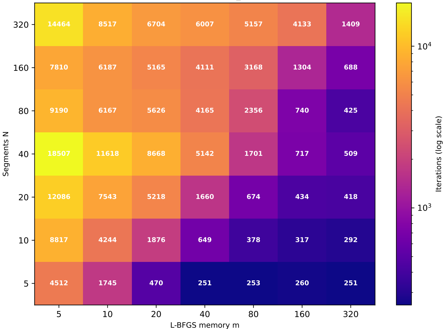
Recurrence T \approx 19.56 (target T=20 , rec_id=98) [49/49 converged]
