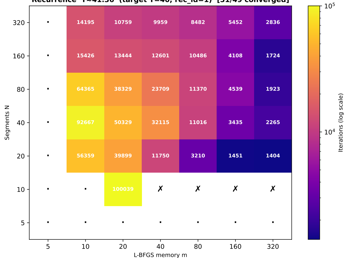
Recurrence T \approx 41.36 (target T=40 , rec_id=1) [31/49 converged]
