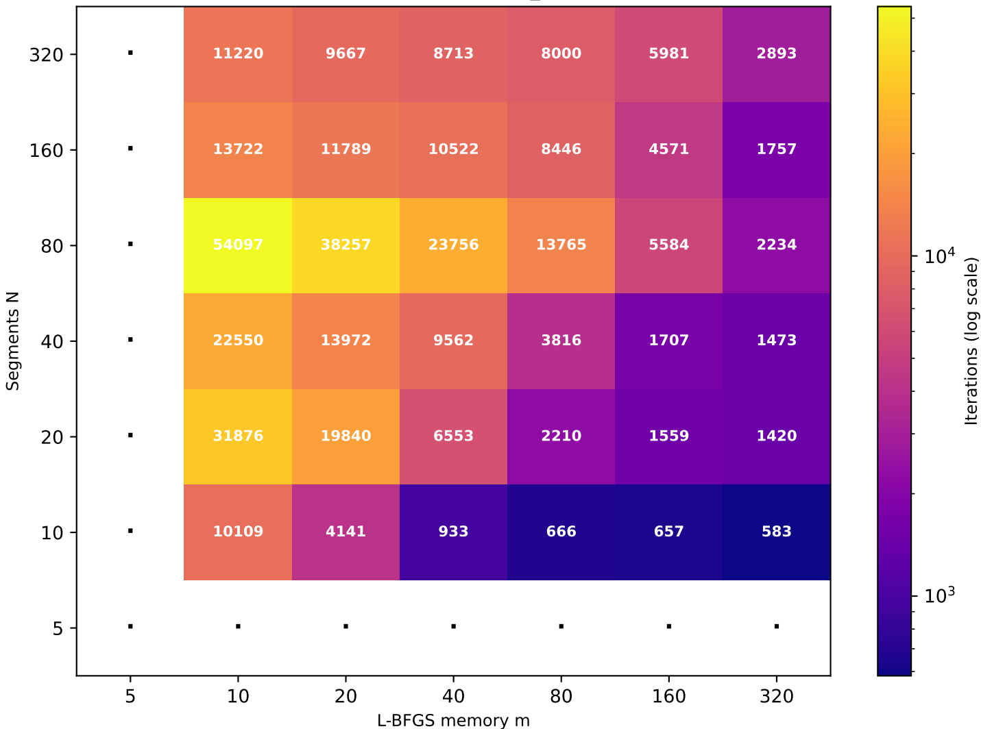
Recurrence T \approx 41.49 (target T=40 , rec_id=4) [36/49 converged]
