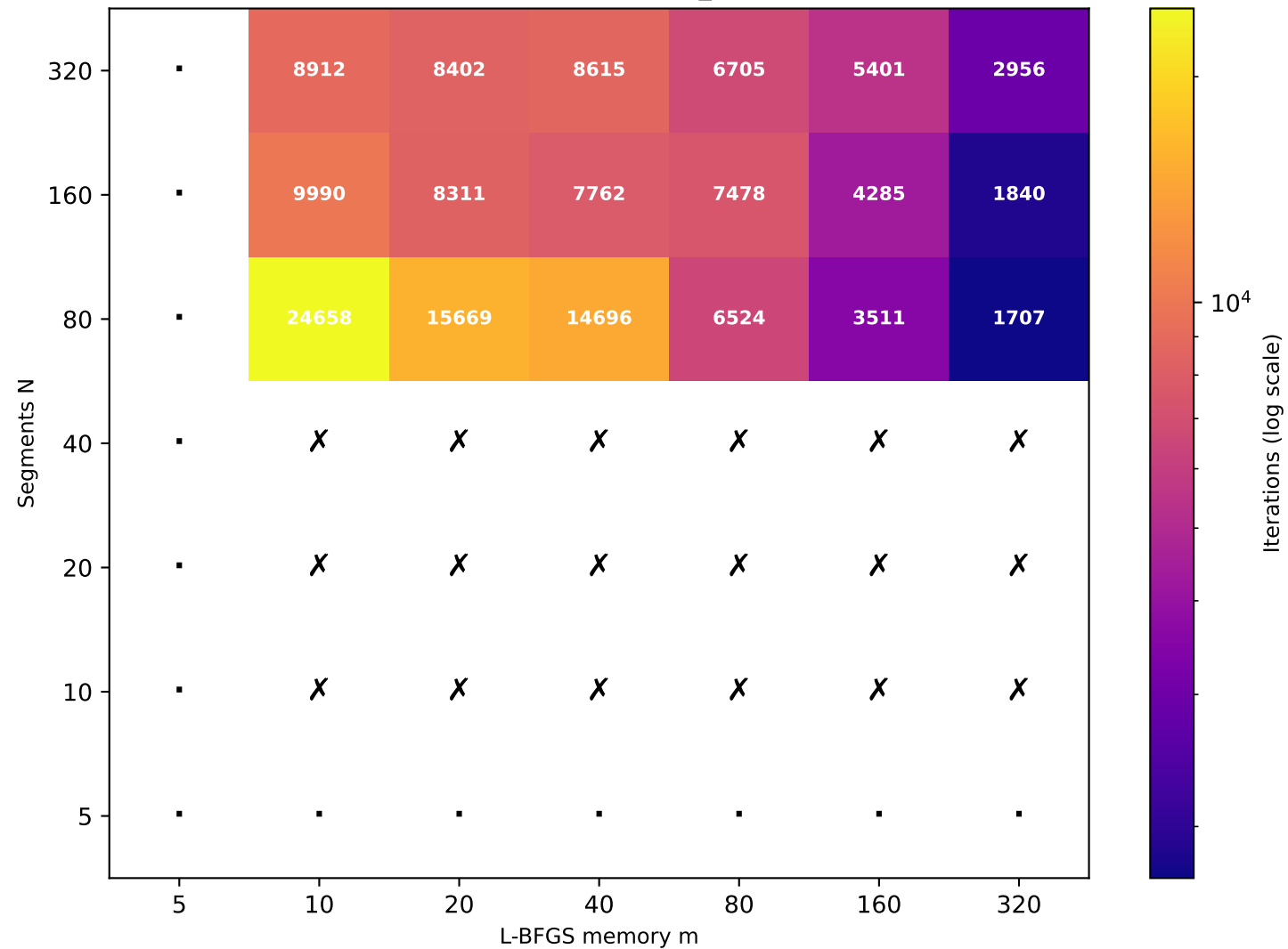
Recurrence T \approx 41.07 (target T=40 , rec_id=6) [18/49 converged]
