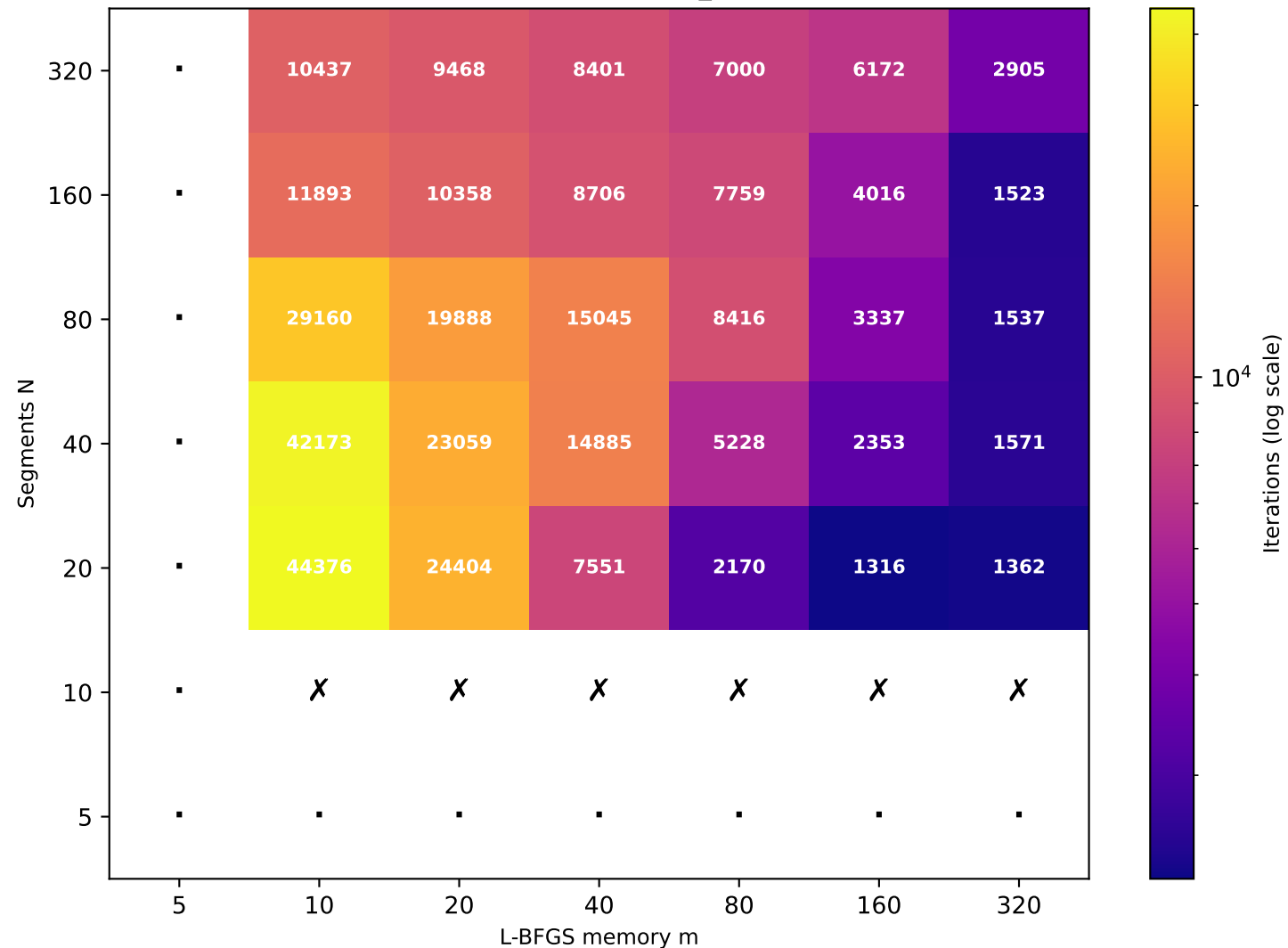
Recurrence T \approx 39.81 (target T=40 , rec_id=7) [30/49 converged]
