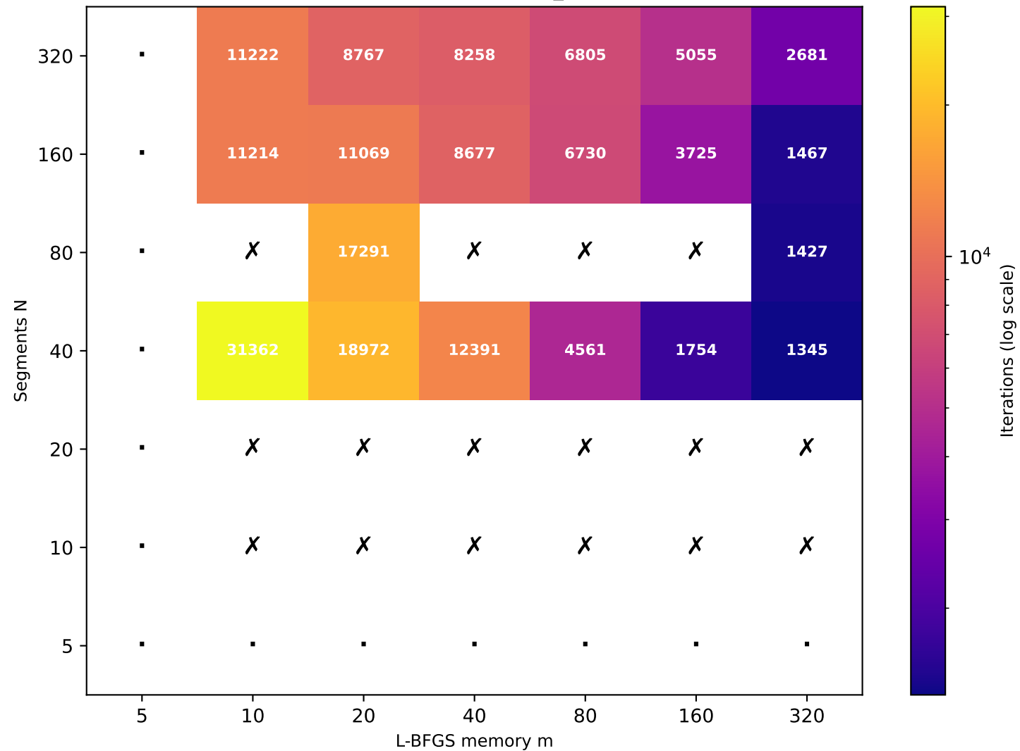
Recurrence T \approx 39.88 (target T=40 , rec_id=8) [20/49 converged]
