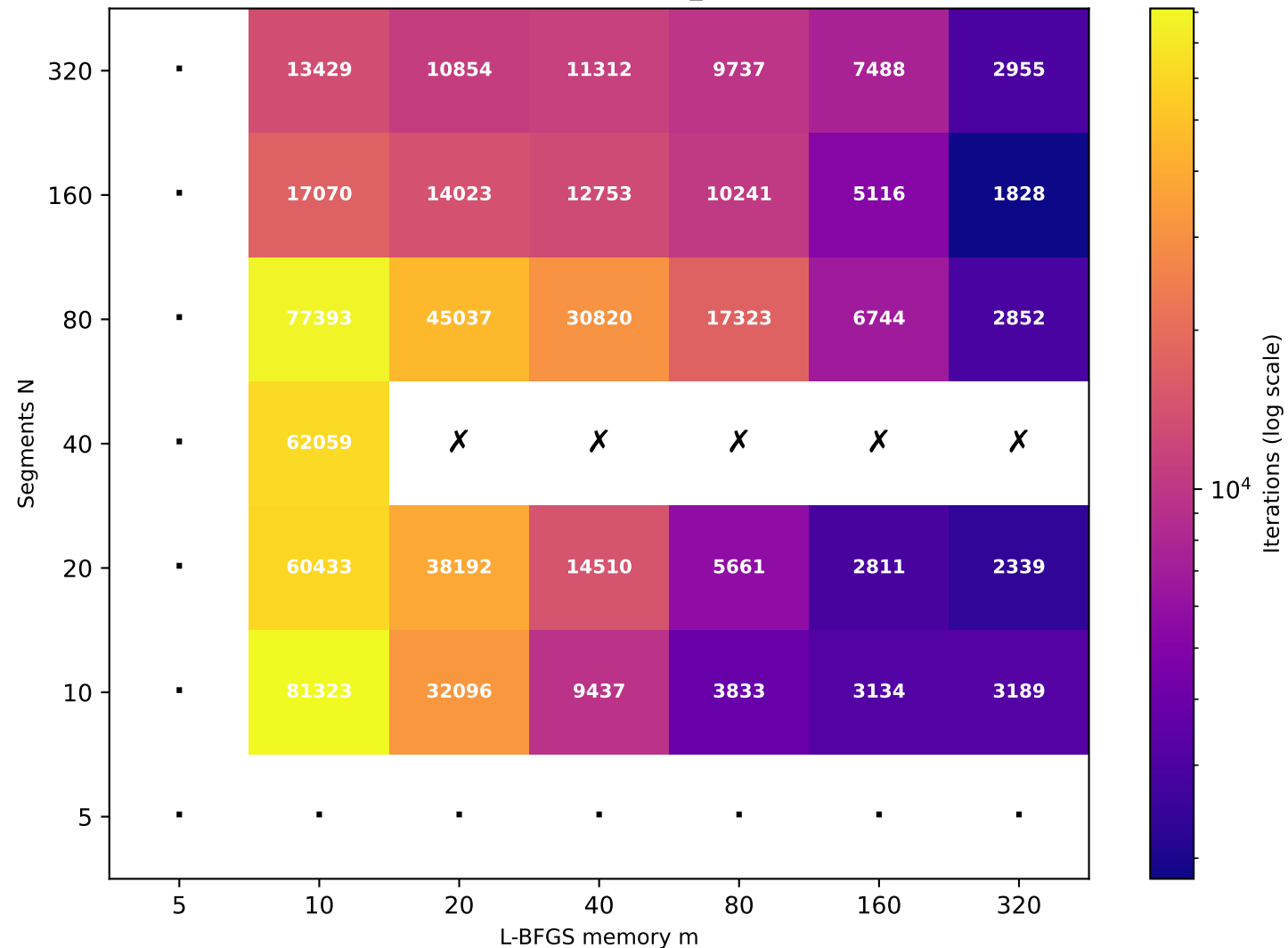
Recurrence T \approx 40.91 (target T=40 , rec_id=13) [31/49 converged]
