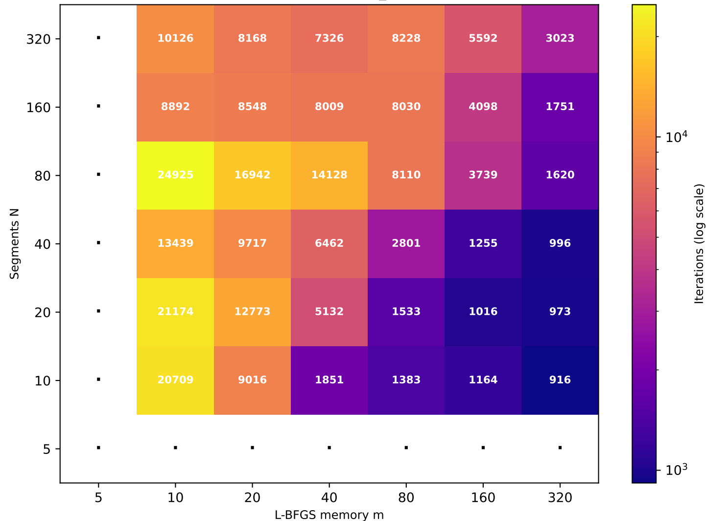
Recurrence T \approx 41.05 (target T=40 , rec_id=14) [36/49 converged]
