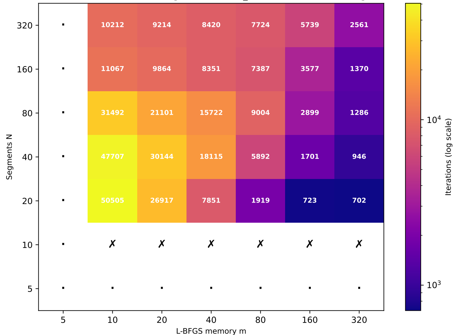
Recurrence T \approx 38.07 (target T=40 , rec_id=15) [30/49 converged]
