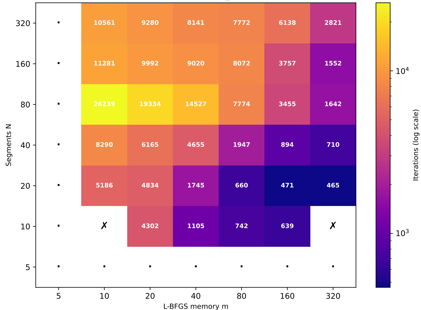
Recurrence T \approx 40.80 (target T=40 , rec_id=18) [34/49 converged]
