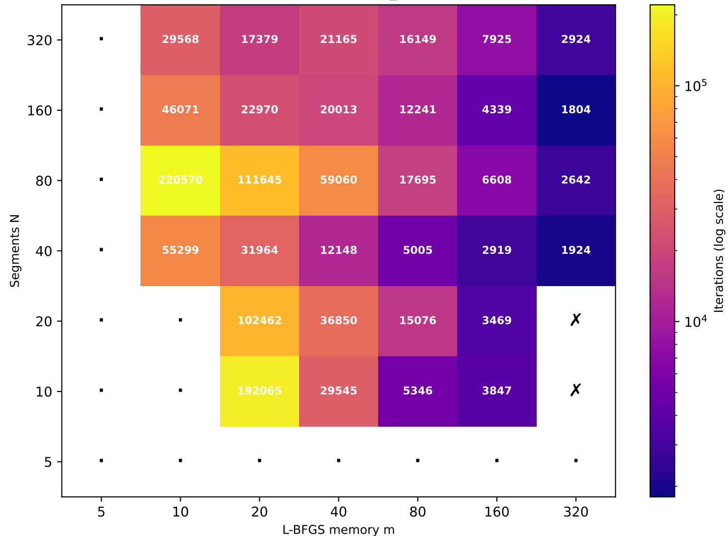
Recurrence T \approx 38.34 (target T=40 , rec_id=19) [32/49 converged]
