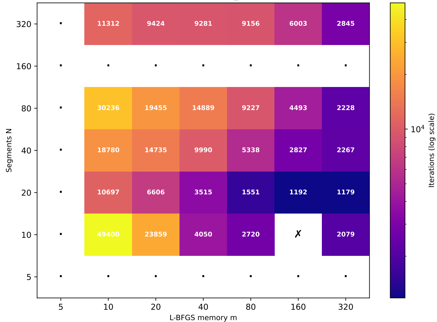
Recurrence T \approx 38.81 (target T=40 , rec_id=23) [29/49 converged]
